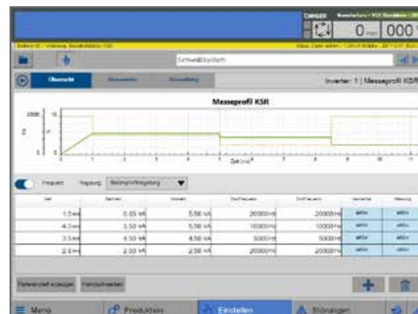
Welding profile with 4 sections and different frequencies
